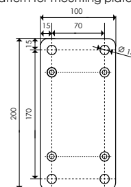
Hole pattern for mounting plate (mm):
