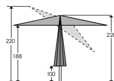
Dimensions (cm) for size 210 x 130 cm:
