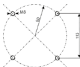
Hole pattern for mounting the umbrella holder:
