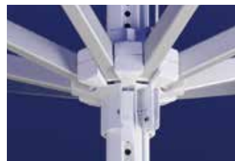
Aluminium frame, cable mechanism, automatic locking handle system
