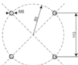
Hole pattern for mounting
