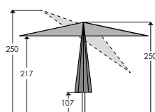
Dimensions (cm) for size 240 x 140 cm:
